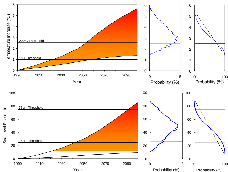
Figure 8.4. The left hand panels show ranges of temperature increase (upper) and sea level rise (lower) 1990–2100 (IPCC 2001), showing a 1^{\circ}\text{C} and 2.5^{\circ}\text{C} warming threshold (upper) and a 25 cm and 75 cm sea level rise threshold (lower). The centre panels show a probability distribution combining two ranges of uncertainty for temperature and sea level rise. The right hand panels show the same probability distributions recast to assess the likelihood of threshold exceedance. The dashed line represents a uniform probability distribution (all points equally likely in the central panels). These charts shows the probability of threshold exceedance manages input uncertainties in a far more robust manner than the prediction paradigm, represented in the centre panels, as it less sensitive to changes in the probability distribution.
