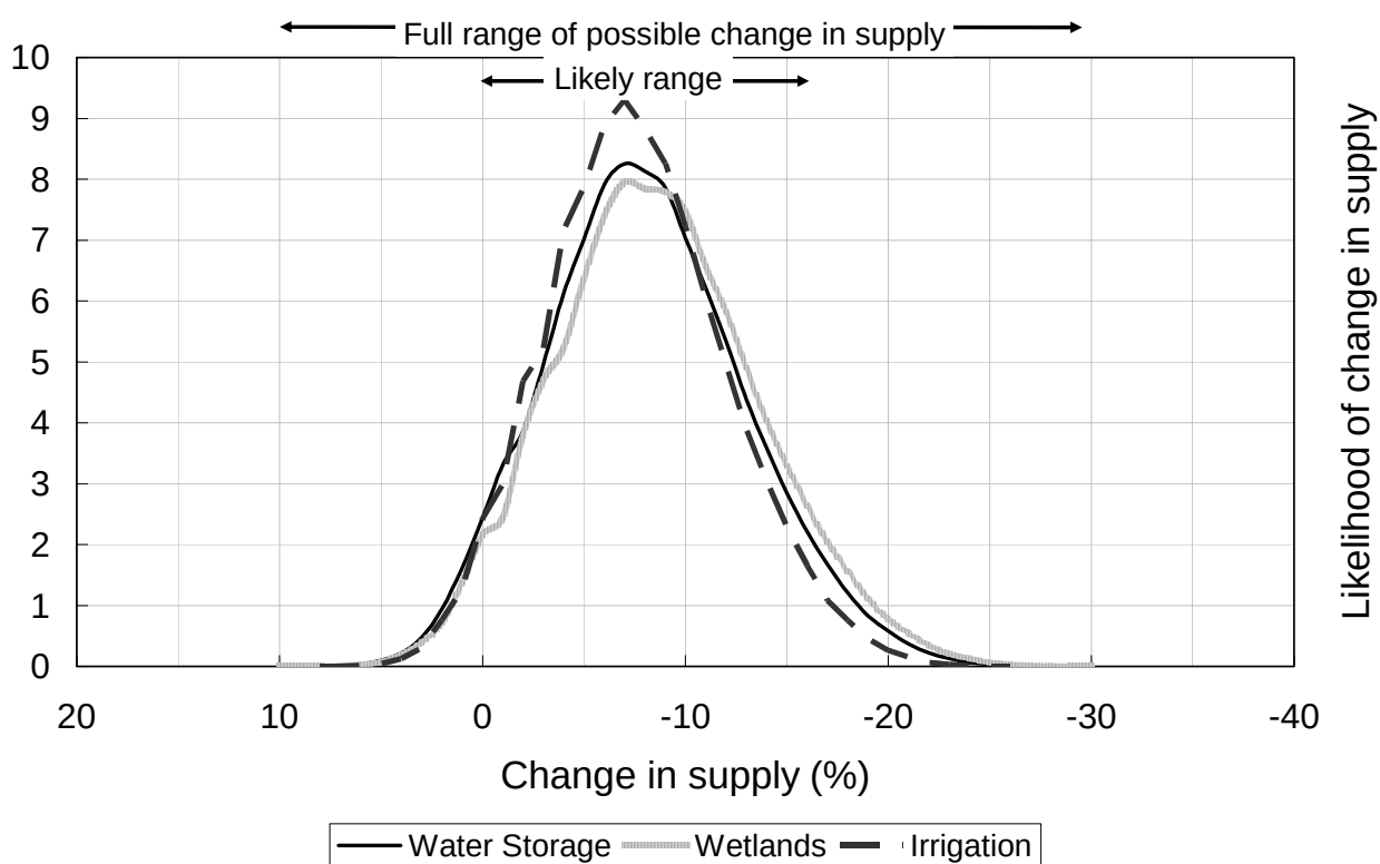
Figure 8.6. Likelihood (%) of changes to mean annual water supply, Macquarie Marsh inflows and irrigation allocations for the Macquarie catchment in 2030
