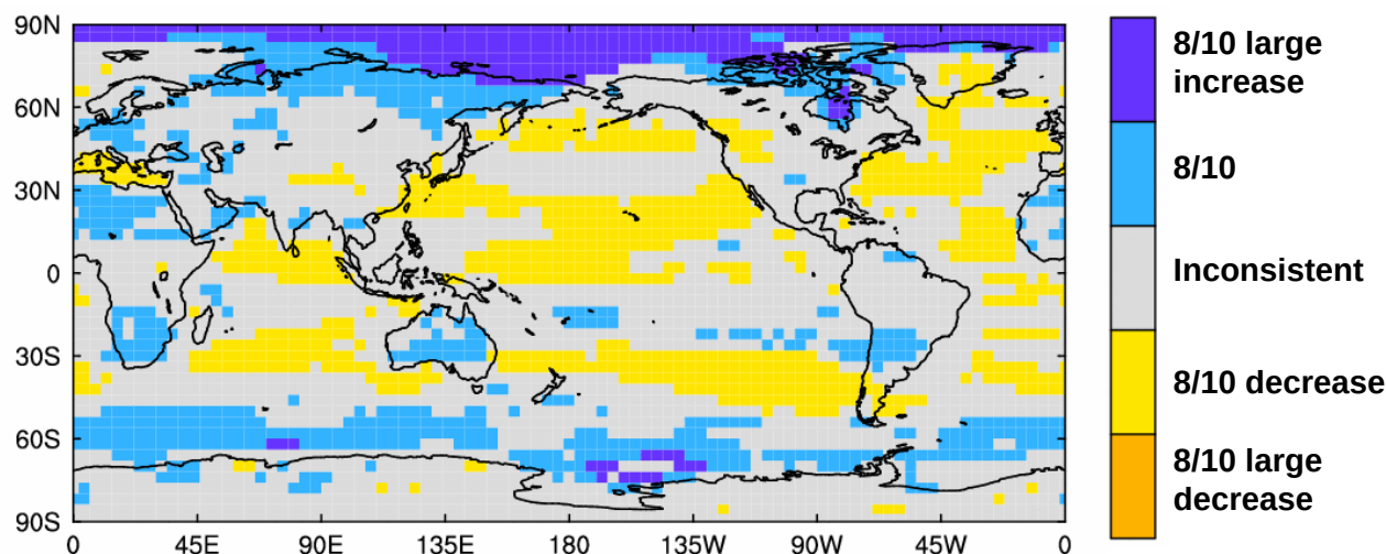
Figure 5.1. Agreement between ten models in the direction of simulated annual near-surface wind change. Large changes are defined as greater than 3 % per °C of global warming.
