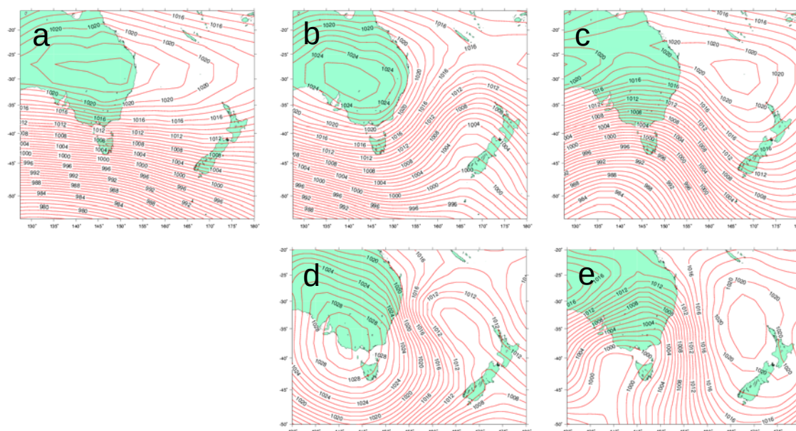
Figure 6.3. (a) the dominant synoptic pattern identified in the Mark3 model accounting for 59 % of winter half-year extreme wind days; (b) and (c), two other synoptic classes in Mark 3 which are similar to two patterns identified in the observations (d) and (e) but high-lighting the tendency in Mark 3 for patterns to be more zonal in structure and for the anti-cyclones to be situated further to the north.
