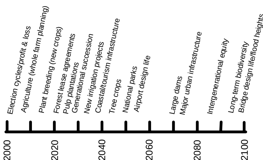
Figure 8.3. Planning horizons relevant to climate risk assessments.
